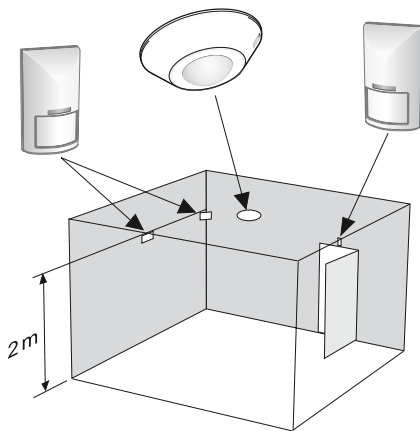
Figure 4. Suitable locations for the DETECT O room unit.
