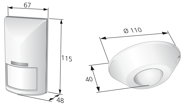
Figure 6. DETECT O V110 and DETECT O T360.
