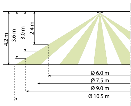
Figure 3. Detection area. Ceiling mounted DETECT O T360.
