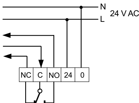
Figure 1. Wiring diagram. NC-C is closed if no occupant is present, NO-C is closed if an occupant is present.
