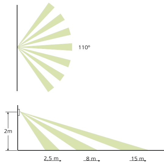
Figure 2. Detection area. Wall mounted DETECT O V110
