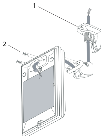
Figure 5. Installation of the DETECT O V110 with supplied mounting bracket (1).
