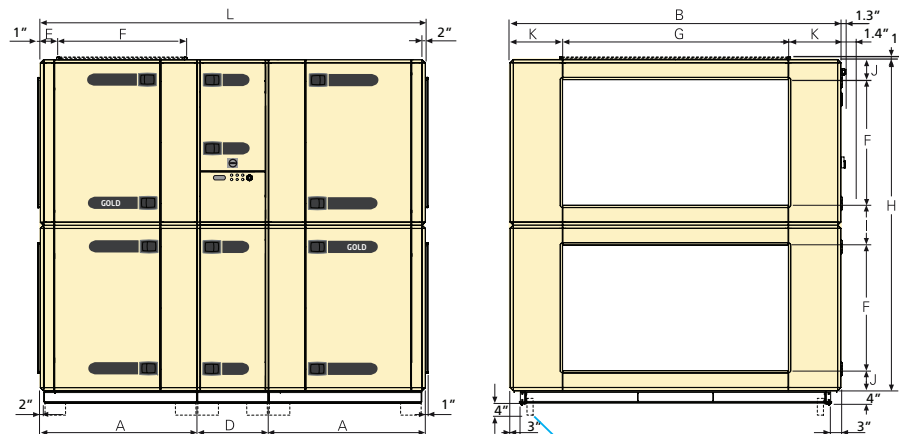
The air handling unit is supplied without end connection panel if a duct accessory housed in an insulated casing will be connected.
