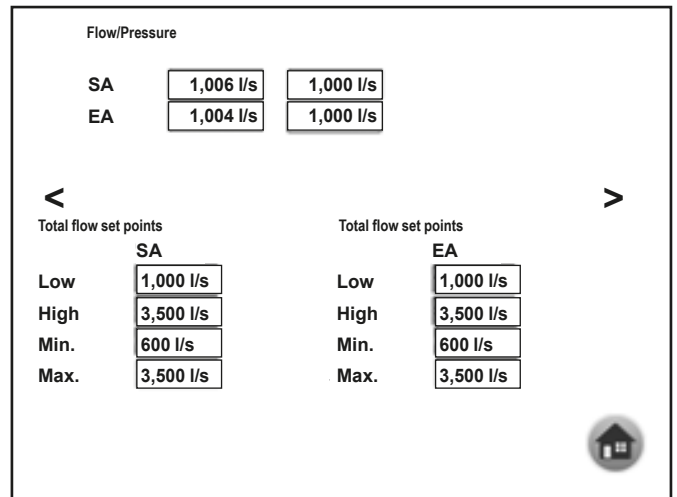
Flow regulation
